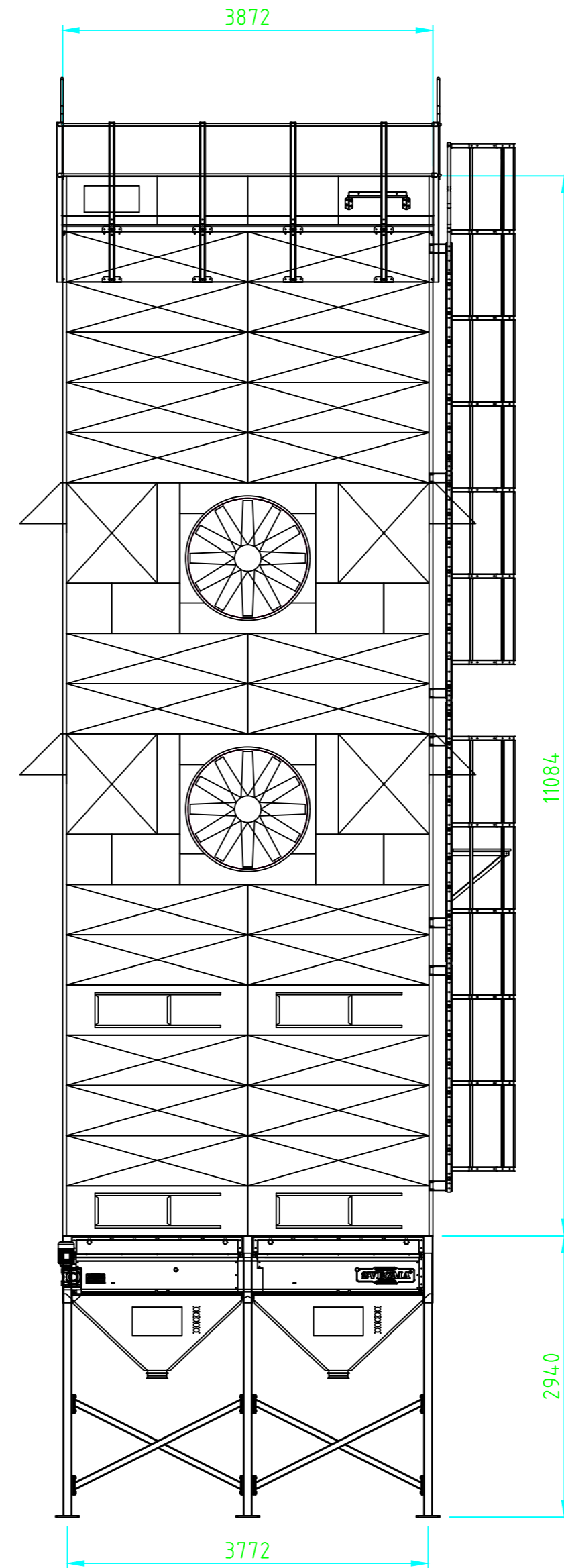
Front view
