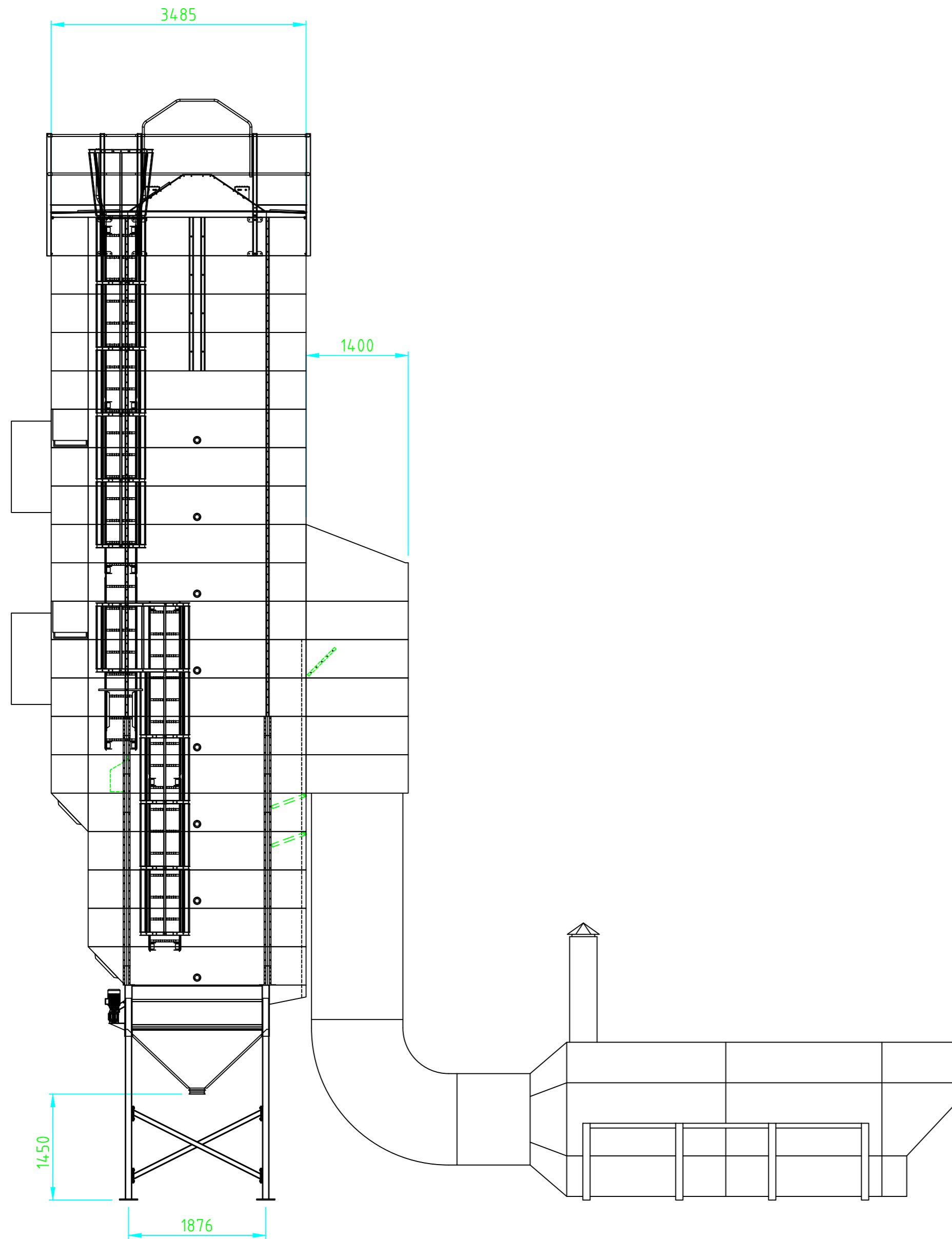
Side view
